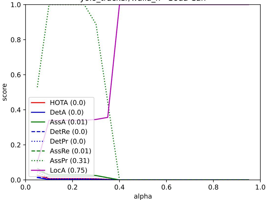
yolo_tracker/walia_n - Soda Can
